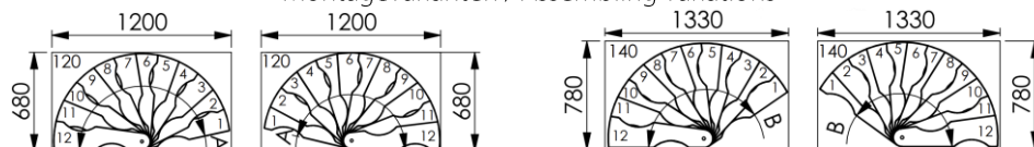
Montagevarianten / Assembling variations
