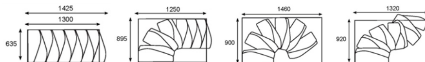
Montagevarianten / assembling options
